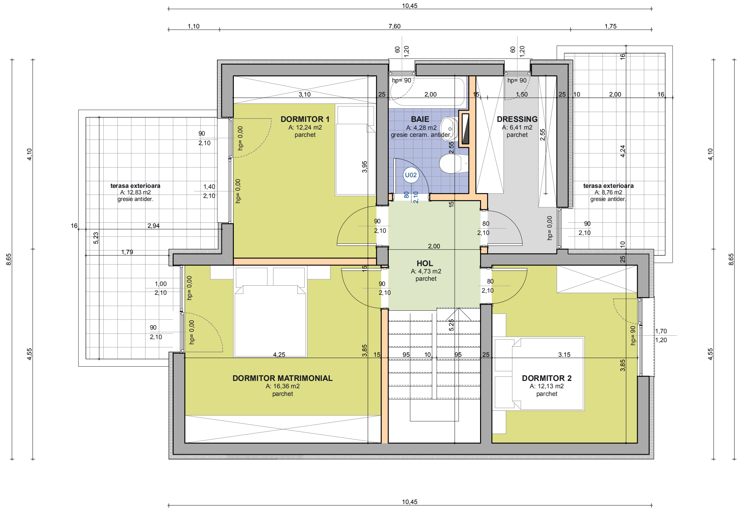
PLAN MANSARDA
